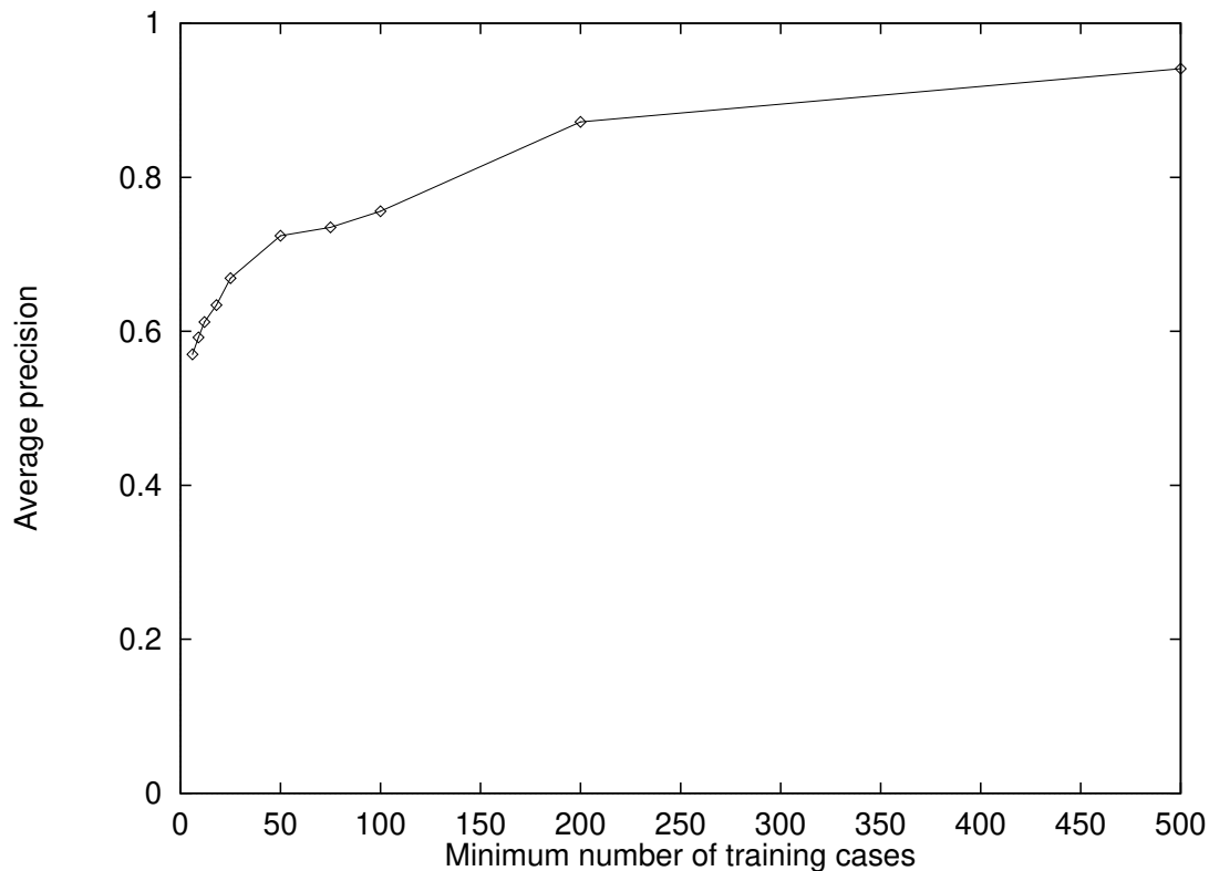
Figure 4: Average precision as a function of minimum number of training examples
