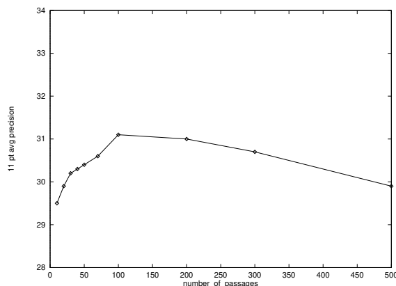
Figure 4: Performance curve of local context analysis on TREC4
