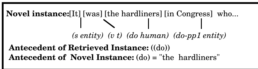
Figure 3: Instance Retrieval
