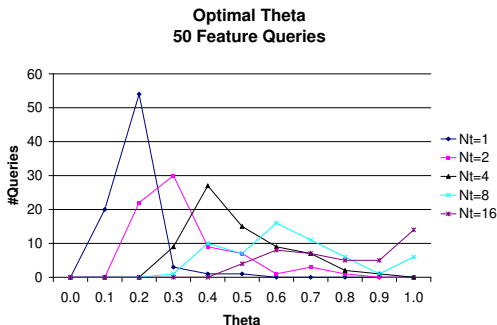
Figure 3: Distributions of optimal threshold parameter \theta for varying Nt .
