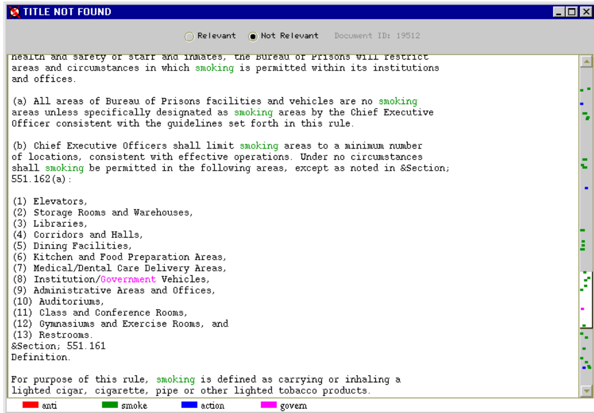
Figure 2. Scrollbar-based visualization
