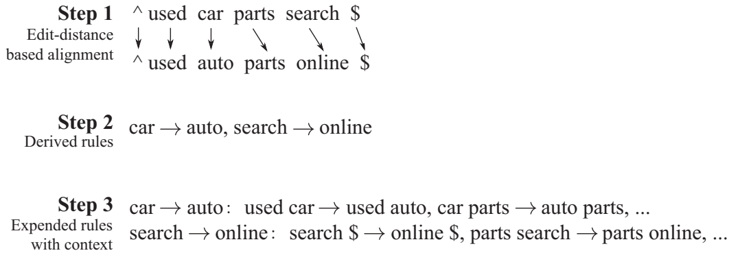
Figure 3: Rule extraction example.
