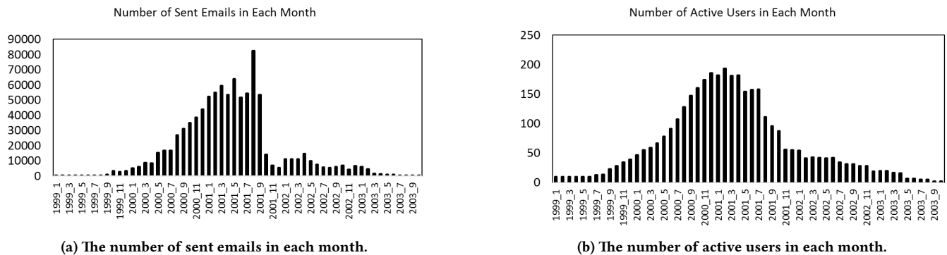
Figure 2: Temporal analysis of the number of sent emails and active users in each month of the Avocado email collection.
